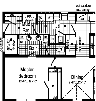
Optional End Entry Utility with 4'x6' Walk-In Tile Shower Note: Living Room size changes to 18'-8" x 12'-10".
