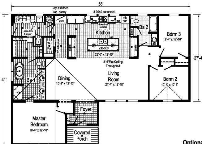
Optional Attic Stairs Requires Optional Expanded Walk-In Pantry Due to Ridge Beam Span
